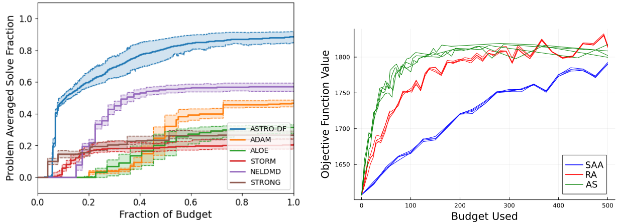
(a) The solvability profile (% of 60 problems from SimOpt library, solved to 0.1-optimality) of ASTRO-DF compared to SAA-based solvers signifies advantage of AS across problems.
